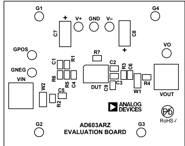
Figure 54. Component Side Silk Screen
