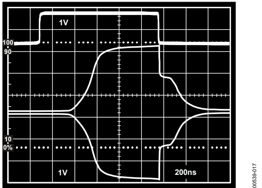
Figure 17. Gain Control Channel Response Time
