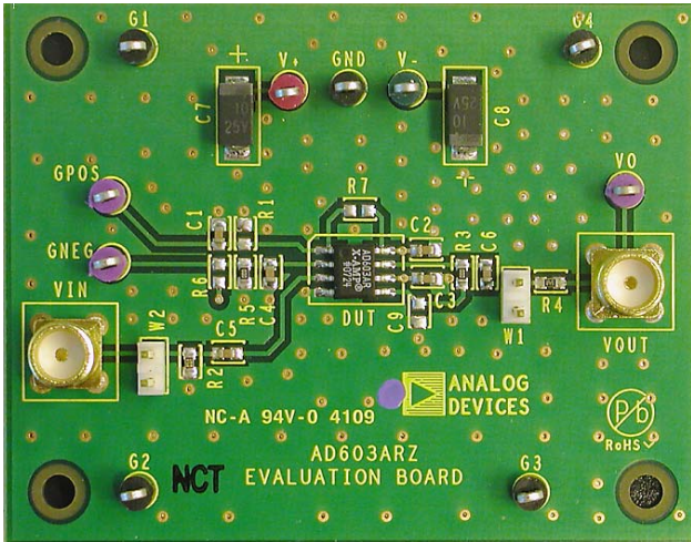
Figure 48. AD603 Evaluation Board
