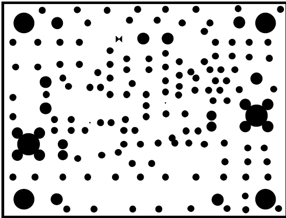
Figure 53. Inner Layer Power Plane
