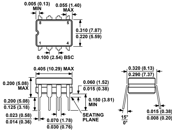
Figure 55. 8-Lead Ceramic Dual In-Line Package [CERDIP] (Q-8)
