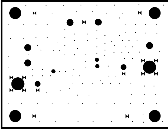
Figure 52. Inner Layer Ground Plane
